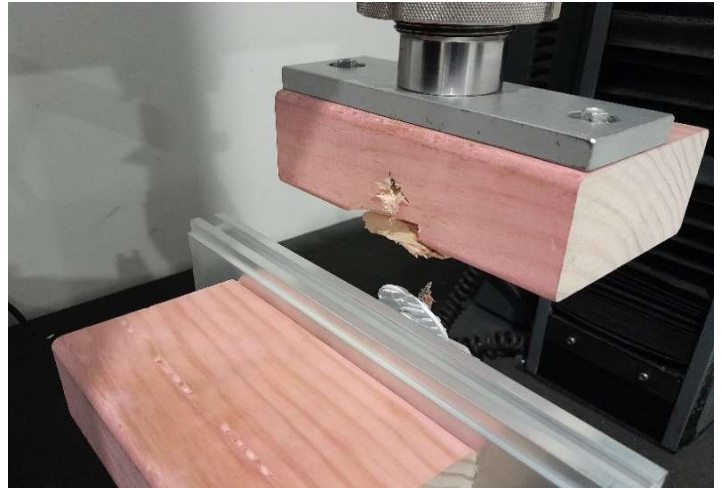
Figure 9 - Pull-out of 8G screw from timber substrate
