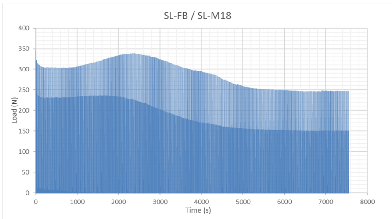
Figure 12 - Graphical representation of the SL-FB / SL-M18 clip set pull-out test
