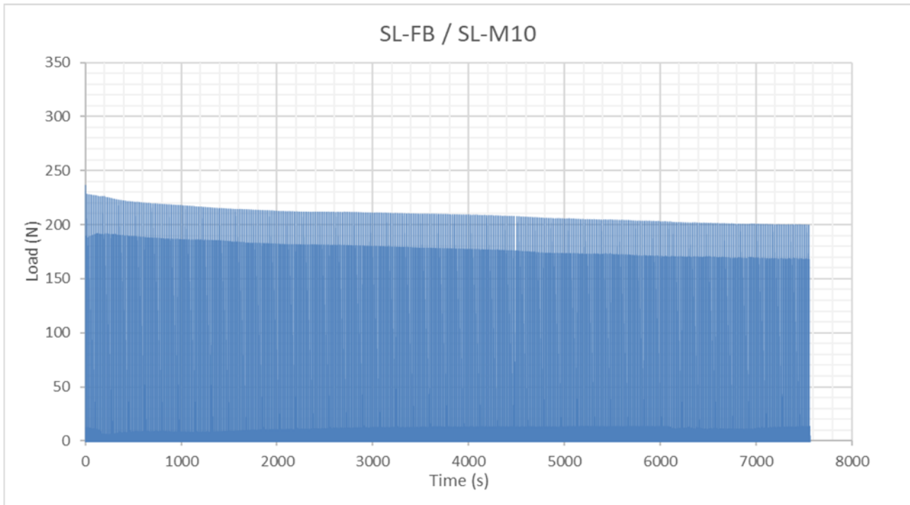
Figure 11 - Graphical representation of the SL-FB / SL-M10 clip set pull-out test
