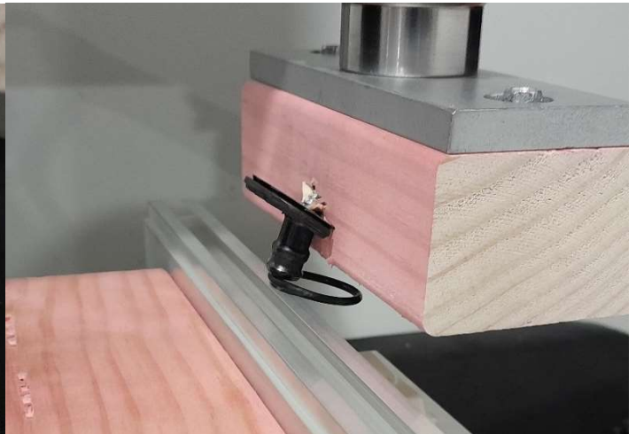
Figure 10 - Combined shear failure of the SL-FB-FR and SL-M18-FR clips
