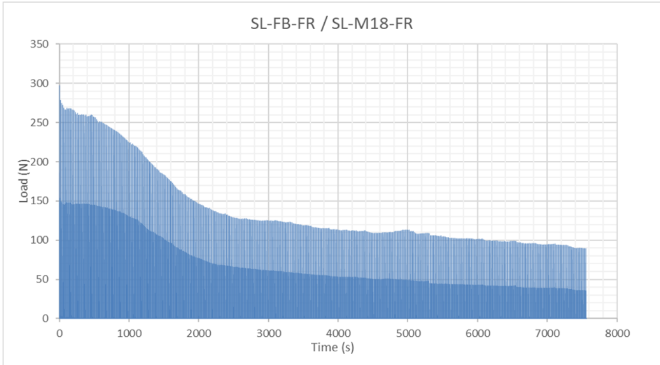
Figure 13 - Graphical representation of the SL-FB-FR / SL-M18-FR clip set pull-out test
